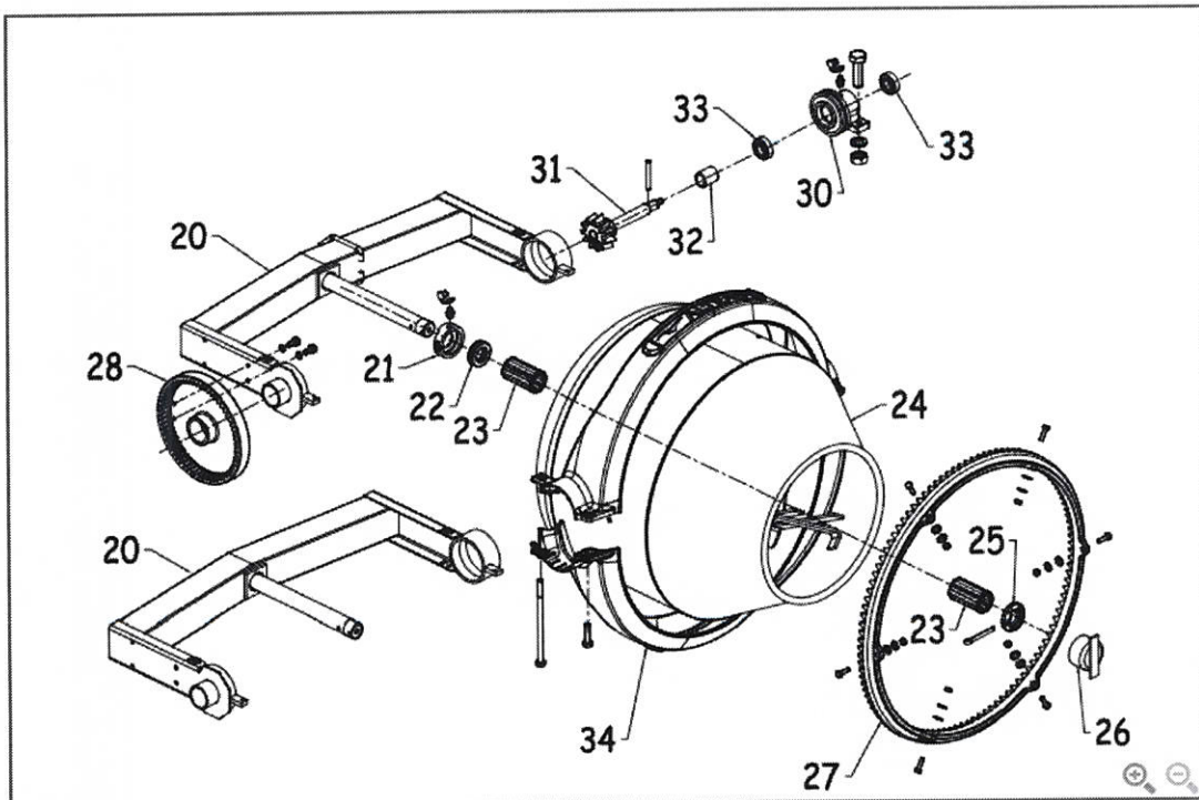
Yoke Drum assembly
